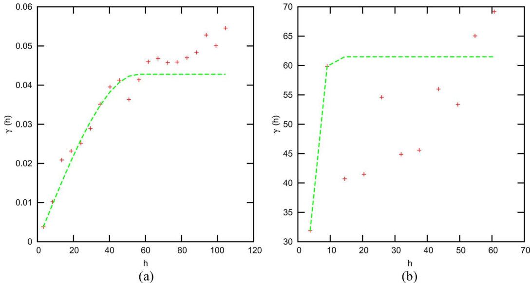
Fig. 2. Semivariograms (+) and (dashed lines) automatically fitted spherical model of (8). (a) Simulated correlated data demonstrating a good fit and (b) degenerate TEC data showing a poor fit.
