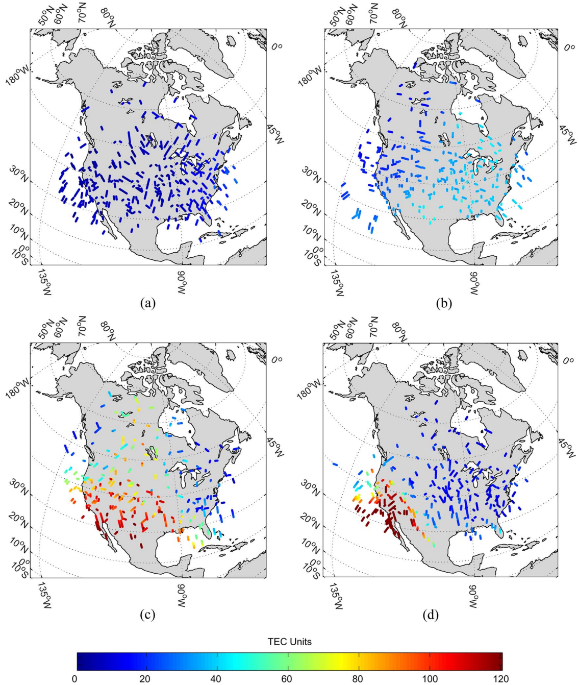
Fig. 8. Example TEC input data for the cross-validation test in Section IV-B. All data are from October 30, 2003 for the time periods (a) 1200–1215 UT, (b) 1600–1615 UT, (c) 2000–2015 UT, and (d) 0000–0015 UT in October 31.
