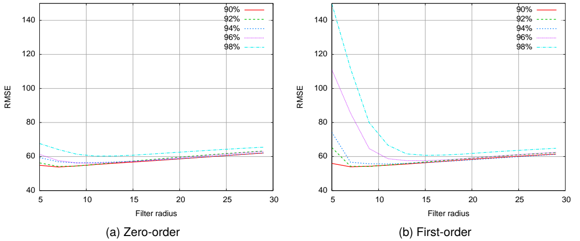
Figure 2.8: Graphs showing RMSE of reconstructions of the crane image from various sparsities and varying filter dimension, using (a) zero- and (b) first-order NC.
